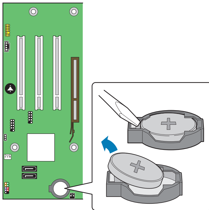
Figure 26. Removing the Battery
